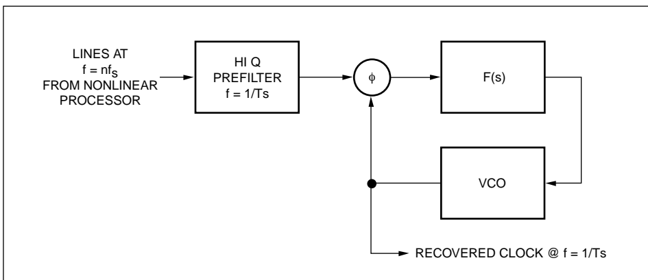
Figure 3. STR narrowband filter employing an analog PLL.
