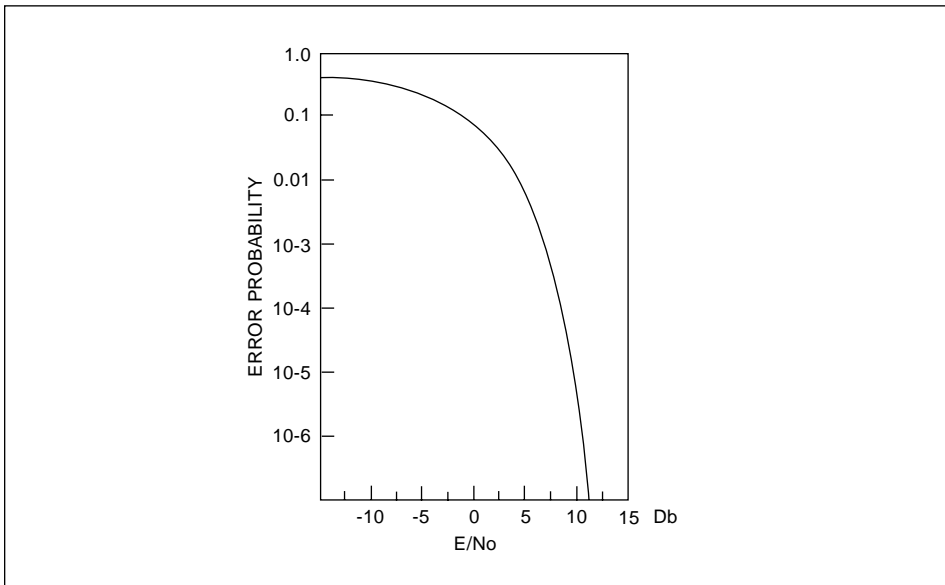
Figure 11. Ideal P(e) curve (BPSK-QPSK)
