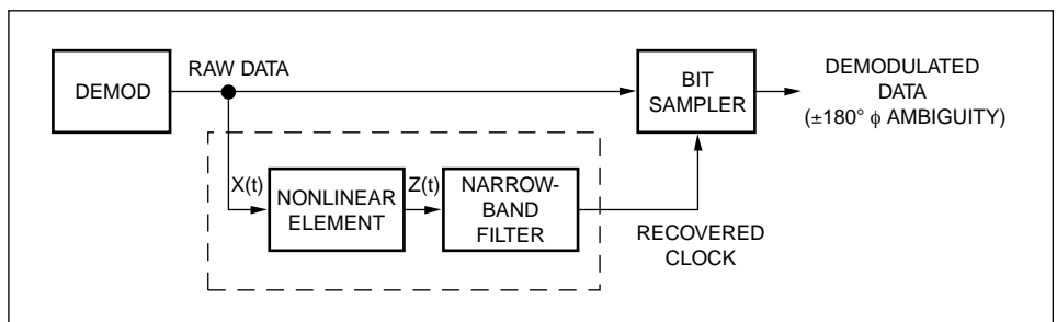
Figure 1. Block diagram of symbol timing recovery.
