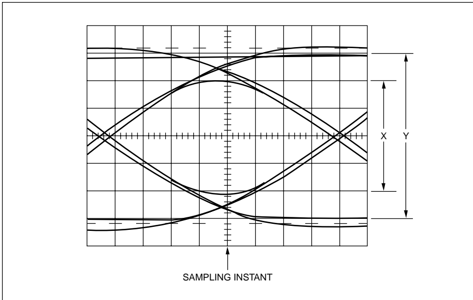
Figure 10. Measured eye diagram of an unequalized filter.
