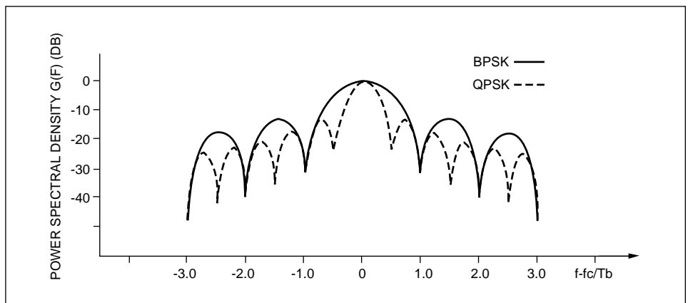
Figure 1. (Part 1) BPSK and QPSK spectra.
