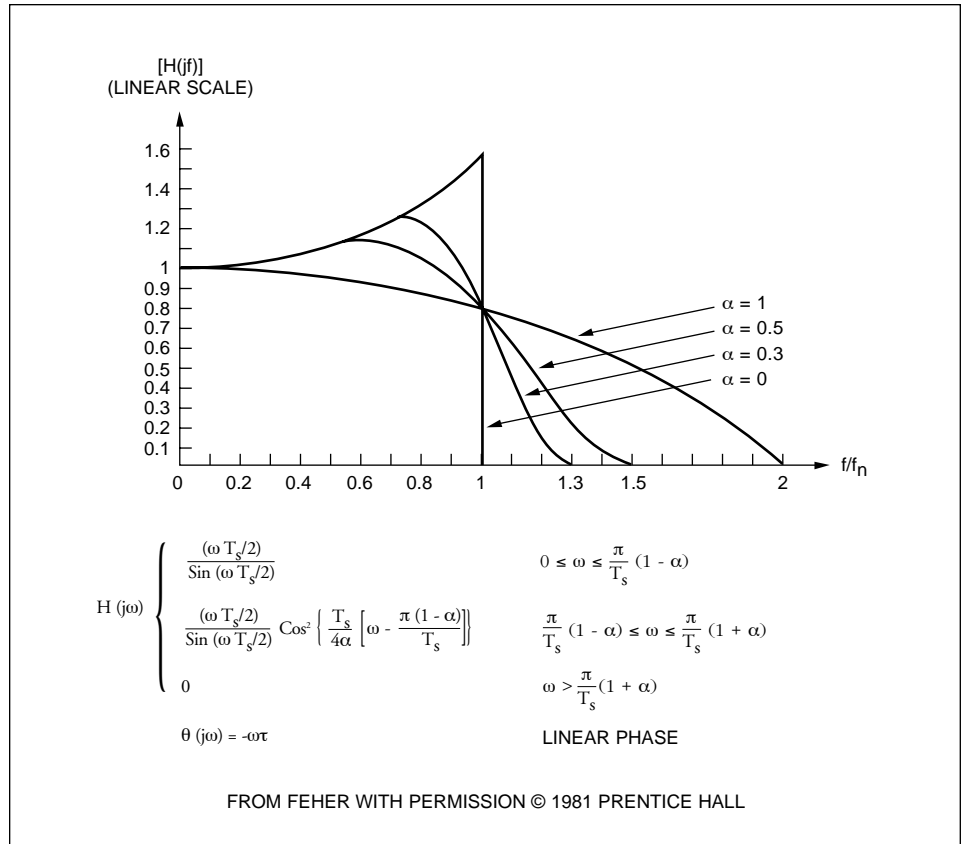
Figure 7. Nyquist channel-pulse transmission.
