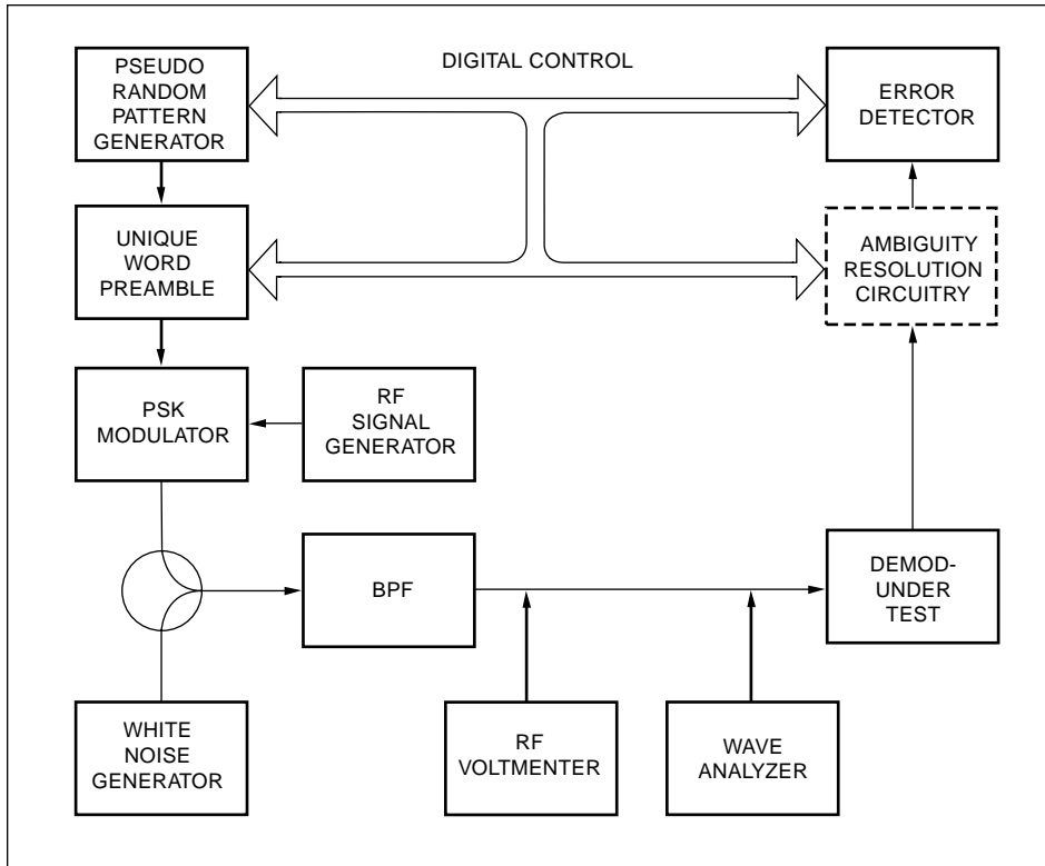
Figure 12. Typical test setup for BER measurement.
