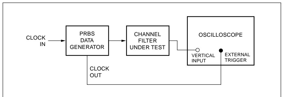
Figure 9. ISI degradation measurement test setup.
