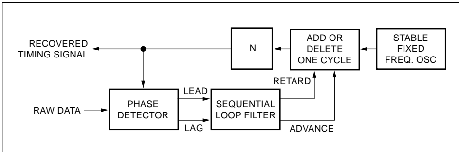
Figure 4A. The (LL)-DPLL.
