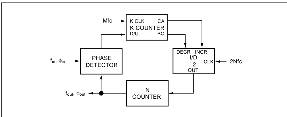
Figure 4B. T.I. SN74LS297 block diagram.
