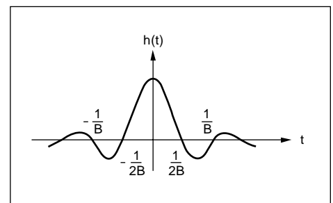
Figure 6A. Desired data channel impulse response.
